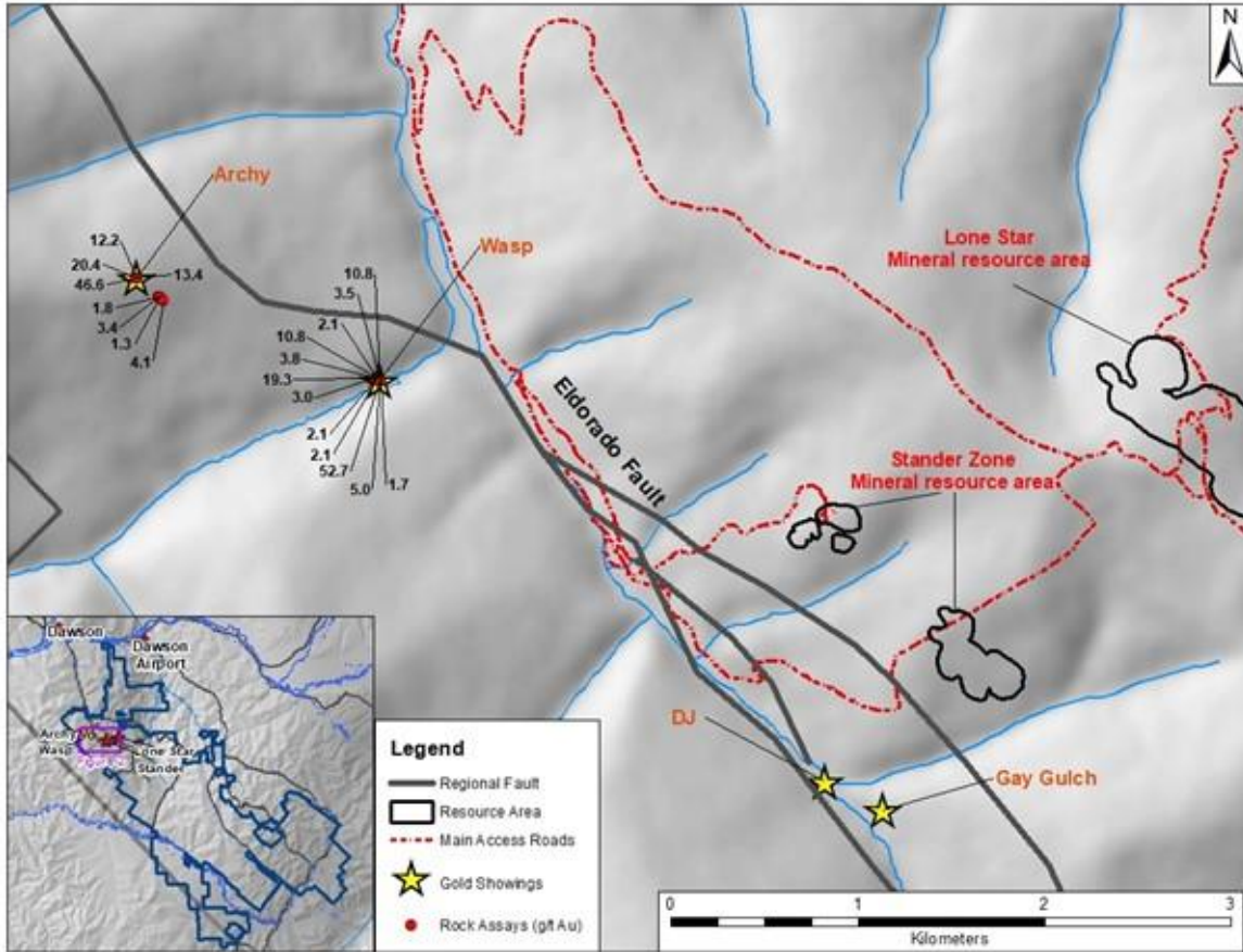
Figure 2: Location of sample assay results (numbers in g/t Au) for Archy and Wasp Showings along the Eldorado Fault.
